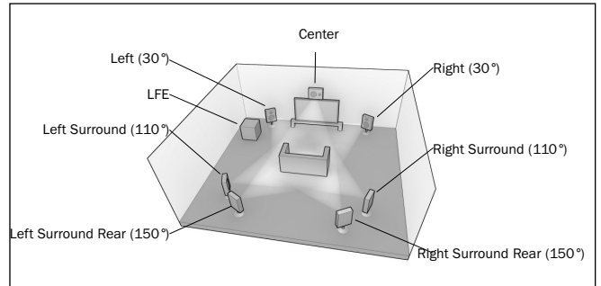
Configuration 6 - 7.1 channel: L, C, R, LFE, Ls, Rs, Lw, Rw
